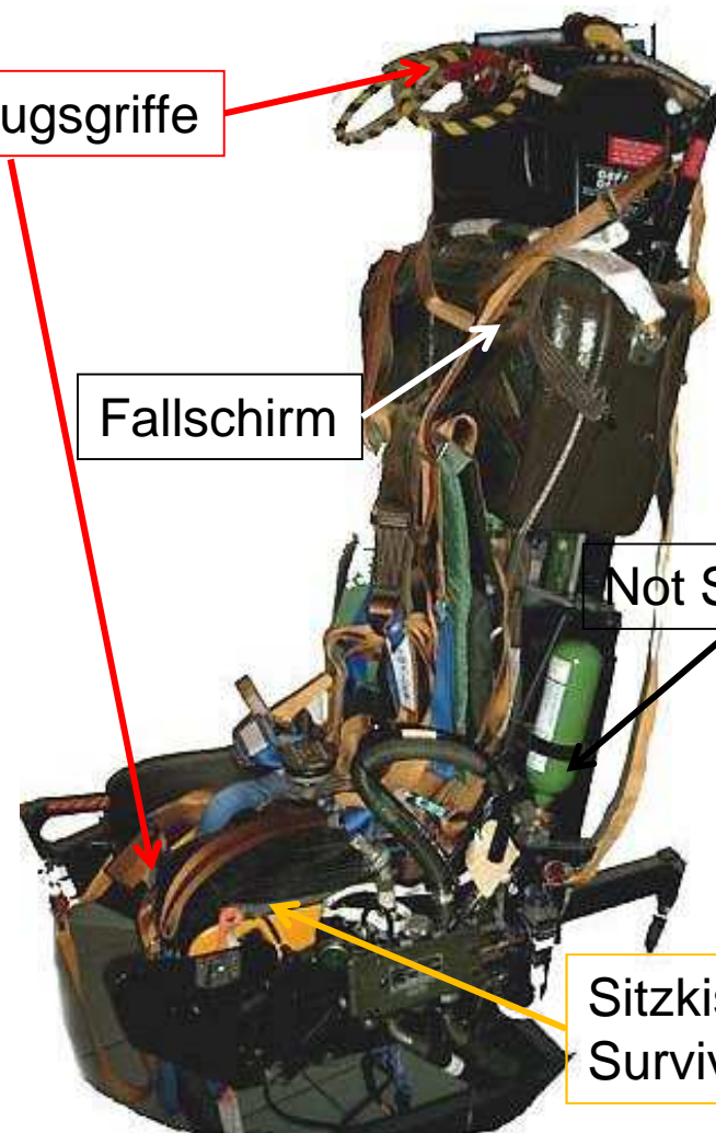
Martin-Baker GQ 7A ab 1967
