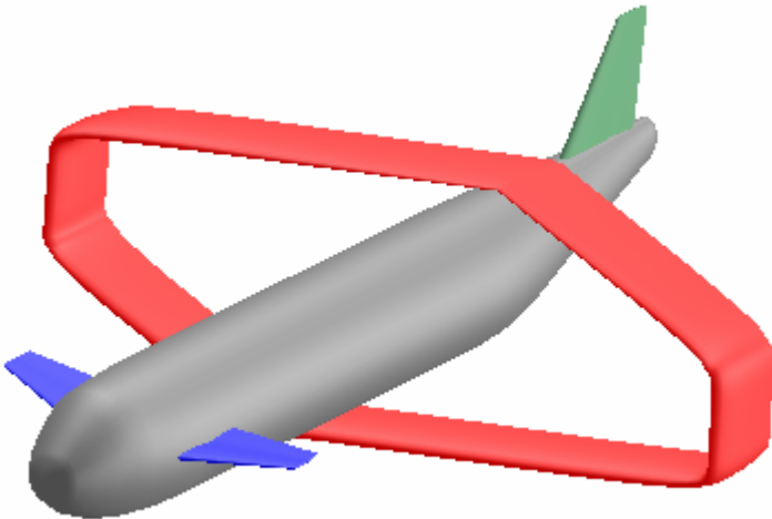
Figure 3.23 “_-, <>, L-H and Can- Aft” Box wing aircraft configuration
