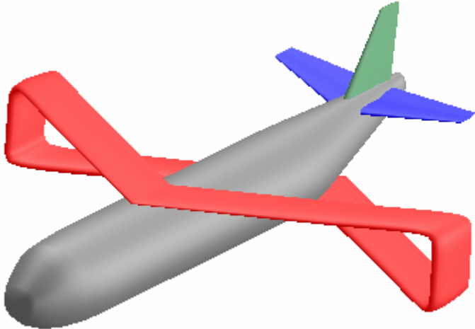
Figure 3.19 “_ , < >, L-H and Aft- Aft” Box wing aircraft configuration
