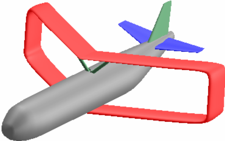
Figure 3.10 “=, <<, L-SH and Aft – Aft” Box wing aircraft configuration
