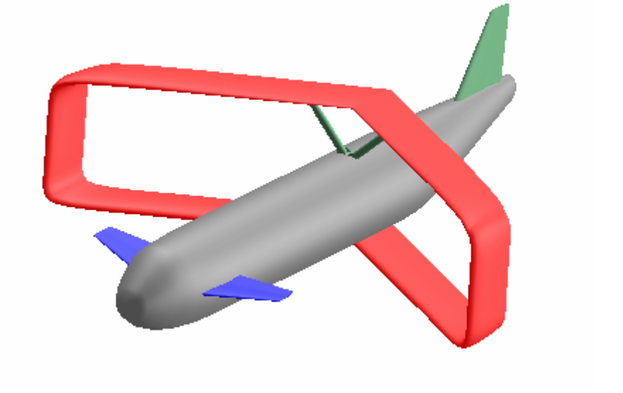
Figure 3.14 “=, >>, L-SH and Can – Aft” Box wing aircraft configuration
