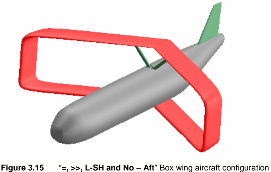
Figure 3.15 “=, >>, L-SH and No – Aft” Box wing aircraft configuration
