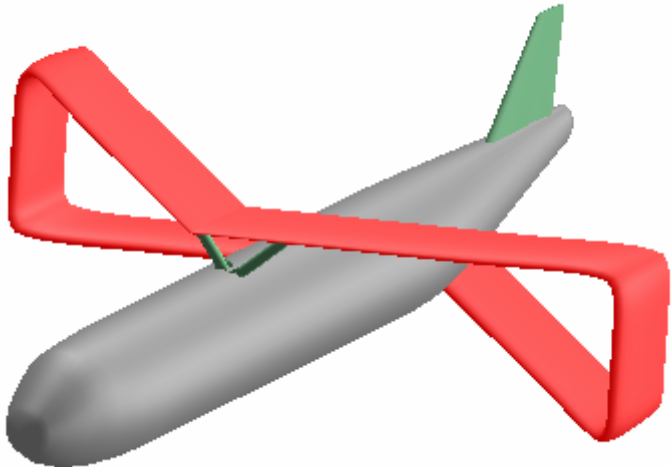
Figure 3.21 “_ , < >, L-SH and No- Aft” Box wing aircraft configuration
