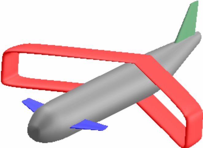
Figure 3.10 “=, <<, L-SH and Aft – Aft” Box wing aircraft configuration
