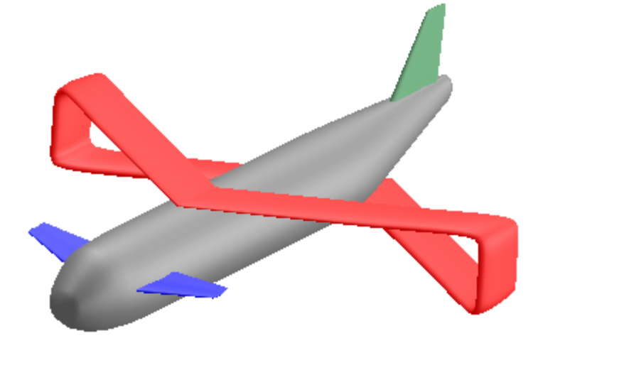
Figure 3.17 “-_, <>, L-H and Can- Aft” Box wing aircraft configuration
