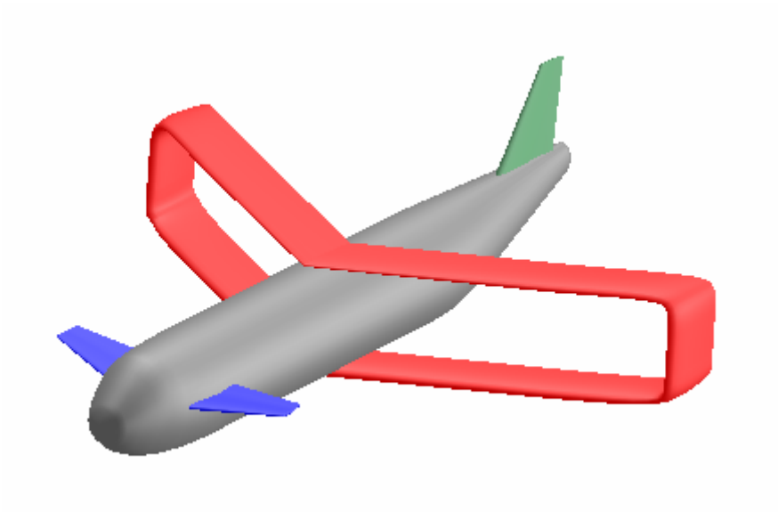
Figure 3.3 “=, <<, L-H and Can – Aft” Box wing aircraft configuration
