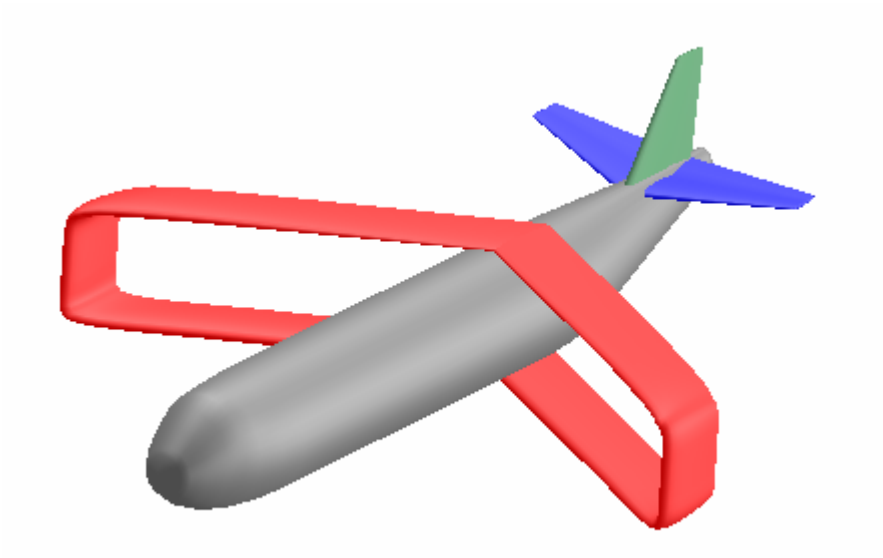
Figure 3.13 “=, >>, L-H and Aft – Aft” Box wing aircraft configuration
